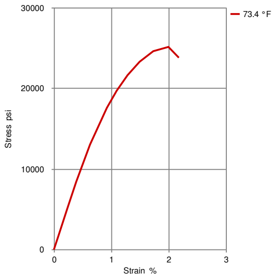
Stress-strain (dry)
