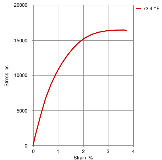
Stress-strain (cond.)
